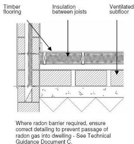
Diagram B14 Suspended timber floor with quilt insulation (Par. B.7.2)
