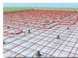
7 Install reinforcing steel mesh according to design. Underfloor heating system can be installed at this stage.
