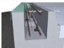
6 Install 5mm U-Sine ties through the ring beam profiles and place steel reinforcing according to supplied design.
